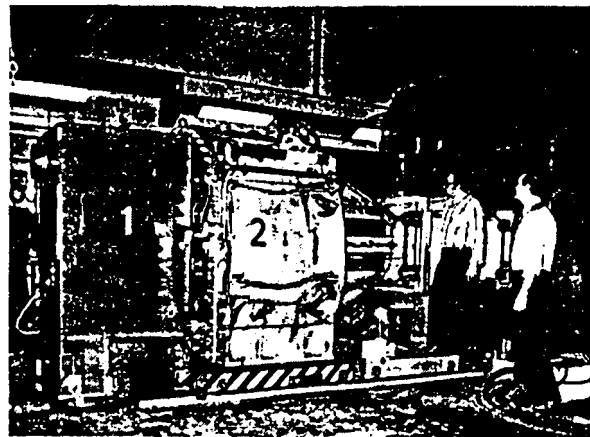
The photograph shows the whole RF system for heavy ions. Between the rotco and the vacuum tank the MFR line is inserted.
