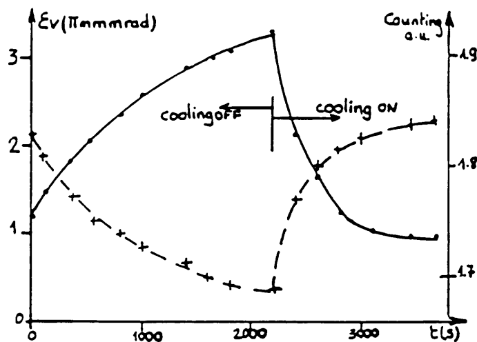
Figure 4 Evolution of the vertical emittance (solid) and elastic counting rate in jet set (dashed) with stochastic cooling ON and OFF at p = 1500 MeV/c and with 18 \cdot 10^9 antiprotons.
