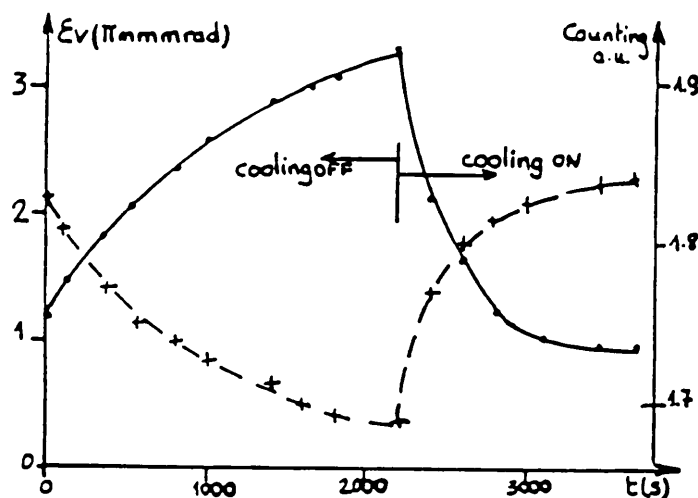
Figure 4 Evolution of the vertical emittance (solid) and elastics counting rate in jet set (dashed) with stochastic cooling ON and OFF at p = 1500 MeV/c and with 18 \cdot 10^9 antiprotons.
