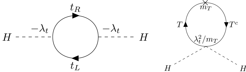
Figure 4: The cancellation between quadratic divergences from the top quark loop and fermionic top-partner loops.
