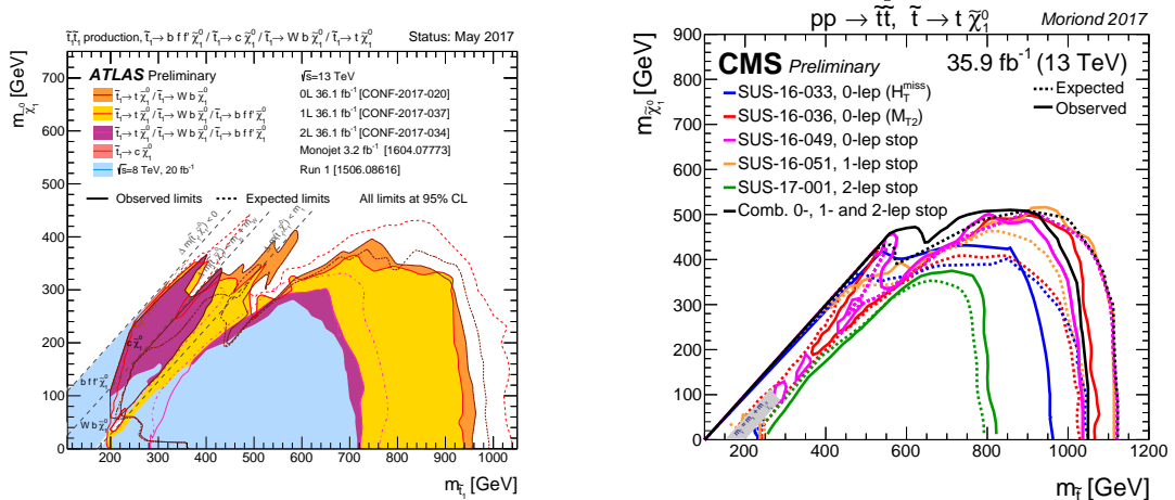
Figure 10: Current experimental limits on a simplified model with stop squarks and a neutralino. These limits are already placing significant pressure on SUSY naturalness for this class of models.
