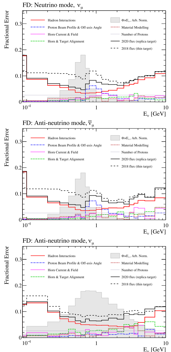
Fig. 6 Uncertainty on the right-sign flux in \nu -mode (top) and right-sign (middle) and wrong-sign (bottom) fluxes in \bar{\nu} -mode, broken down by the sources of uncertainty. The solid black line shows the total flux uncertainty in this analysis, and the dashed black line shows the total uncertainty for the previous T2K analysis [1, 2], which used NA61/SHINE thin target data. The grey shaded region shows the shape of the neutrino flux
