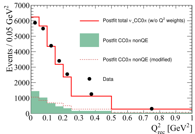
Fig. 39 The ND prediction after the fit to data for the FGD1 \nu_\mu CC0 \pi sample is shown with the data, where the non-CCQE contribution is shown in shaded green. The dotted red line shows the non-CCQE contribution needed for the overall prediction to match the data. The weight is the ratio of the dotted red line to the shaded green
