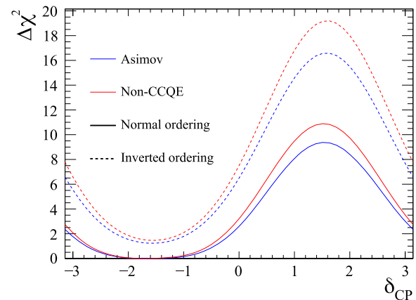
Fig. 41 Comparison of confidence regions in \sin^2 \theta_{23} - \Delta m_{32}^2 (top) for the expected sensitivity fit (blue) and the “non-CCQE” simulated data study (red), and the \Delta\chi^2 as a function of \delta_{CP} (bottom)
