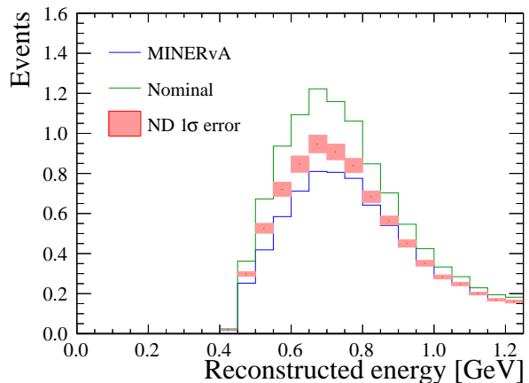
Fig. 43: The predictions for the 1 Re1de selection at the FD using the unchanged model (green) and including the MINERvA pion-suppression (blue). The red bands show the propagated ND prediction from the fit to the simulated data set, with the 1\sigma uncertainty bands.
