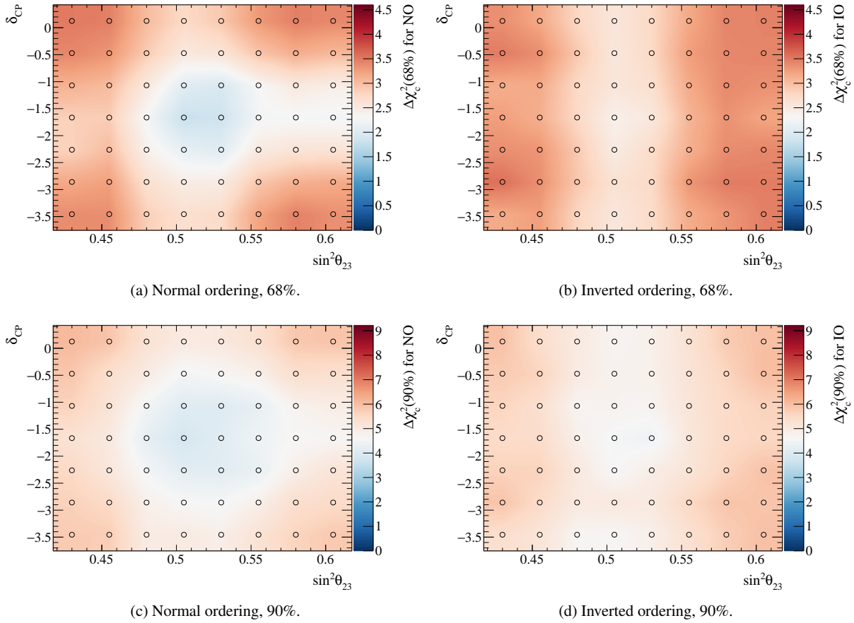
Fig. 47: 68% and 90% FC-corrected critical \Delta\chi^2 values for 2D-fits of \sin^2 \theta_{23} - \delta_{\text{CP}} over both mass orderings, computed at the points indicated by circles and bi-linearly interpolated for the regions in between the points. The colour scheme is chosen to show the asymptotic values from Wilks's theorem in white.
