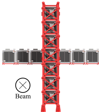
Fig. 2: The INGRID on-axis ND, used to measure the neutrino beam profile and rate [29]. The beam direction is shown as into the paper.
