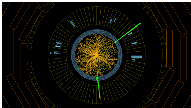
Fig. 2. Visualisation of a proton collision inside the CMS detector leading to a signal of two high-energetic photons (two long green lines). This could either show the signal of a Higgs boson that transformed into two photons or a background event. There is no way to know for sure what has caused a single event, but advanced statistical analyses based on huge amounts of data can help scientists draw conclusions about whether or not the Higgs boson exists. Reproduced from Ref. 29 © CERN ( https://cern.ch/copyright ).
