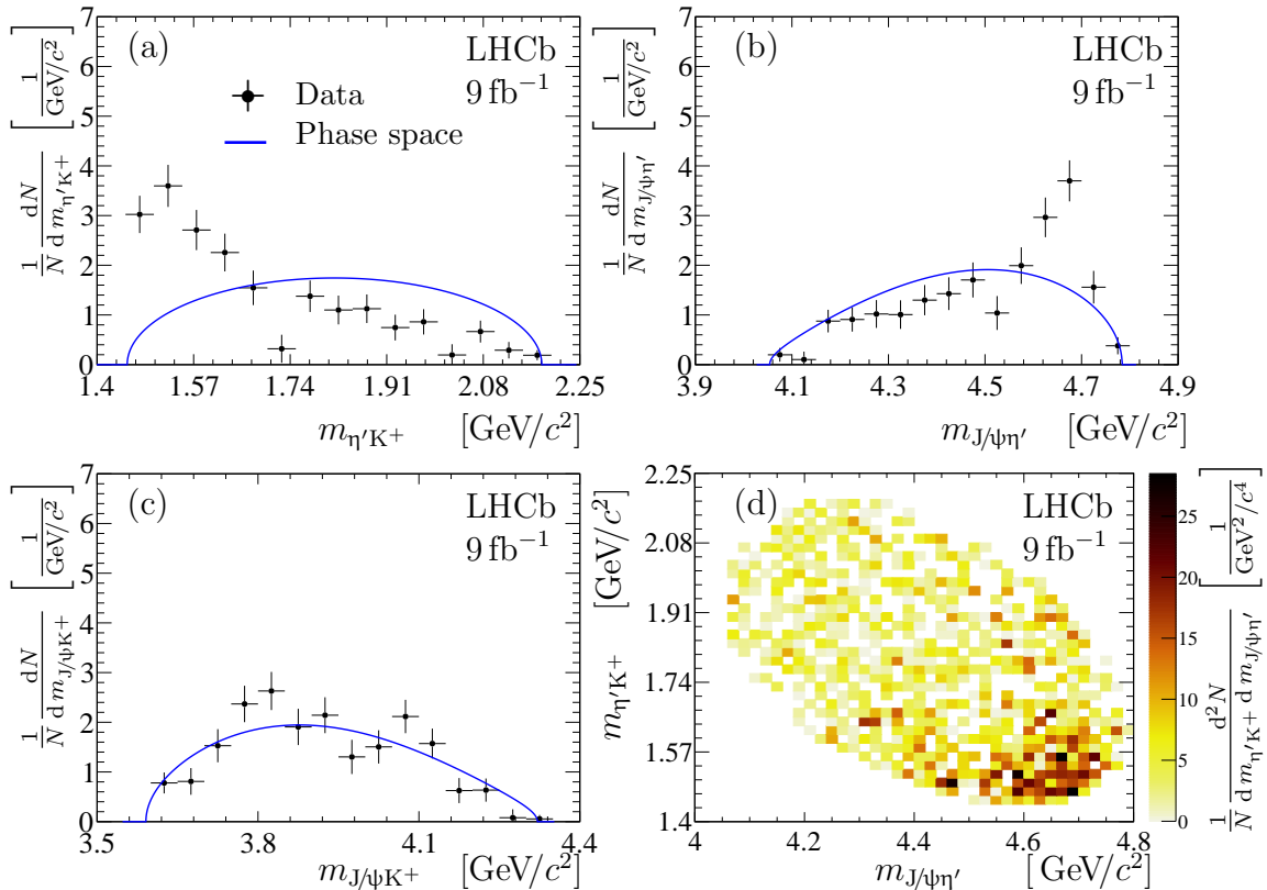
Figure 2: Normalised background-subtracted (a) \eta' K^+ , (b) J/\psi \eta' , (c) J/\psi K^+ mass spectra and (d) two-dimensional mass distribution of \eta' K^+ vs J/\psi \eta' from the B^+ \rightarrow J/\psi \eta' K^+ decays. Superimposed curves are the expectations from a phase-space model.
