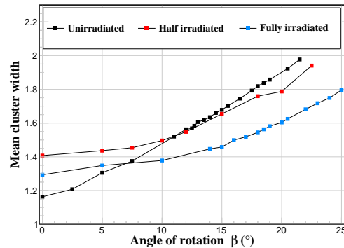
Figure 23: Mean cluster width as a function of incident angle. Results are shown for the correlated sensor of the unirradiated, half irradiated and fully irradiated mini-module.
