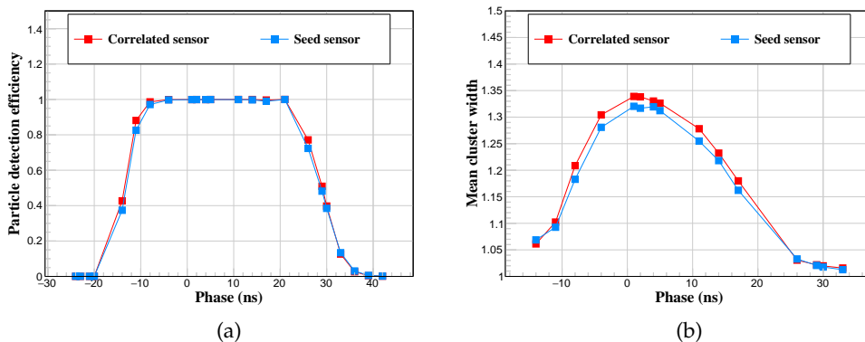
Figure 20: (a) Particle detection efficiency as a function of the clock phase and (b) mean cluster width as a function of the clock phase, for the fully irradiated mini-module.
