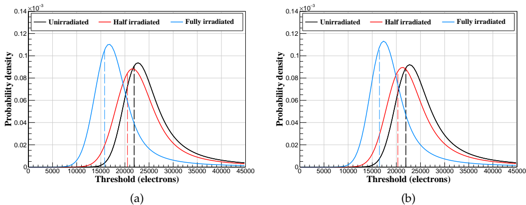
Figure 29: Distributions of the convolution of a Landau function with a Gaussian function, obtained by differentiating the fitting functions to the threshold scans, for the (a) seed sensor and (b) correlated sensor. The dashed lines indicate the Landau functions' most probable value.
