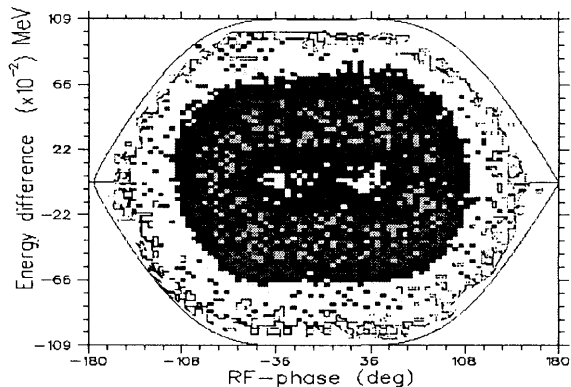
Figure 9: Computer simulation, 105 MeV flat top, V_{16} = 2 kV, 8 ms frequency sweep, intensity 3 \times 10^{12} ppp.
