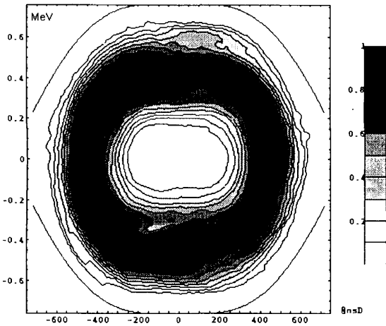
Figure 6: Tomographic reconstruction at 50 MeV, 20 ms filamentation V_{15} = 4 kV, 8 ms sweep, intensity 2 \times 10^{12} ppp.
