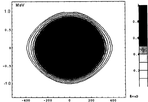
Figure 4: Tomographic reconstruction of phase space after h=1 capture and acceleration to 100 MeV flat top; V_{16}= 2\text{kV} , frequency sweep in 20ms, intensity 7 \times 10^{12} ppp.
