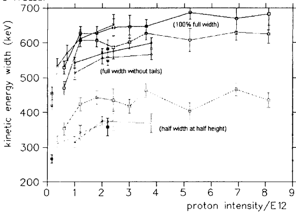
Figure 3: Beam energy width versus injected intensity.
