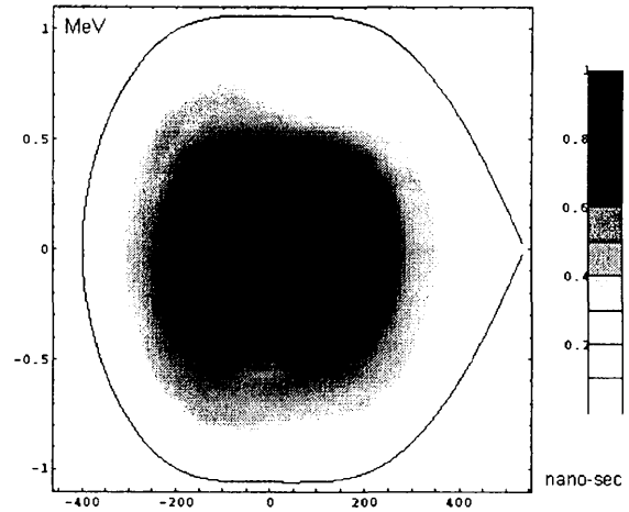
Figure 8: Tomographic reconstruction of phase space at 120 MeV, V_{15} = 4 kV, 6 ms frequency sweep, 10^{12} ppp.
