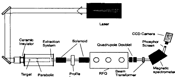
Figure 1: Scheme of the CERN Laser Ion Source
