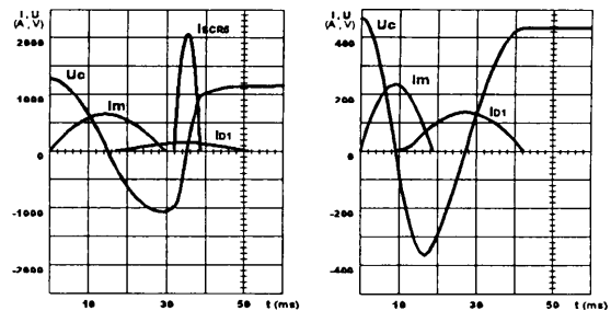
Figure 6: Waveforms of DHPTT02 and DHPTS01.
