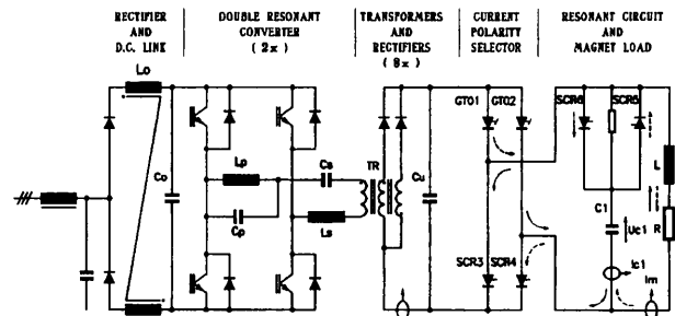
Figure 3: Circuit layout of DHPTT01 power converter.
