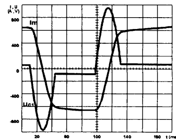
Figure 4: Waveforms of DHPTT01 converter.
