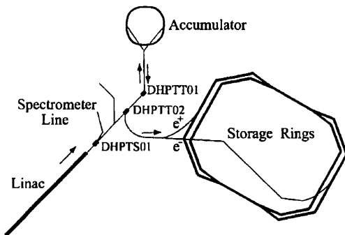
Figure 1: Beam transfer lines with three pulsed magnets.
