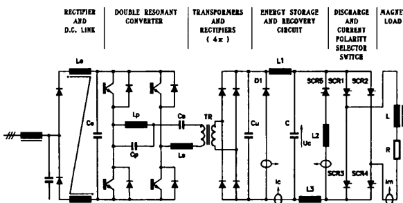
Figure 5: Circuit layout of DHPTT02 power converter.
