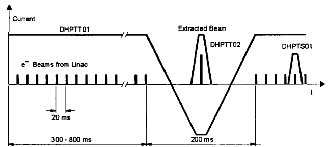
Figure 2: AR beam injection and extraction schemes.
