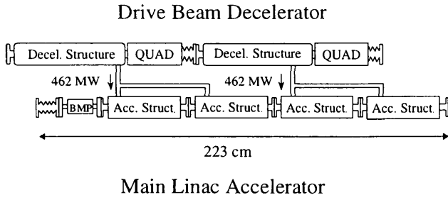
Figure 2: One main beam and drive beam module.
