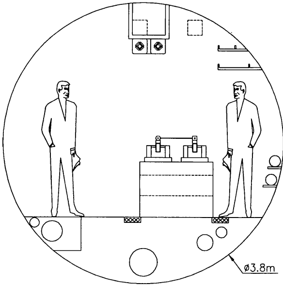
Figure 3: Tunnel cross-section.
