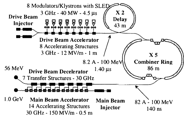
Figure 9: CTF3 schematic layout.
