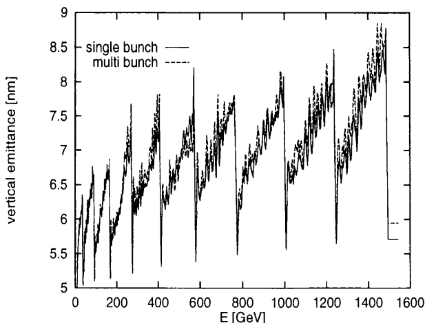
Figure 5: Emittance variation along the main linac.
