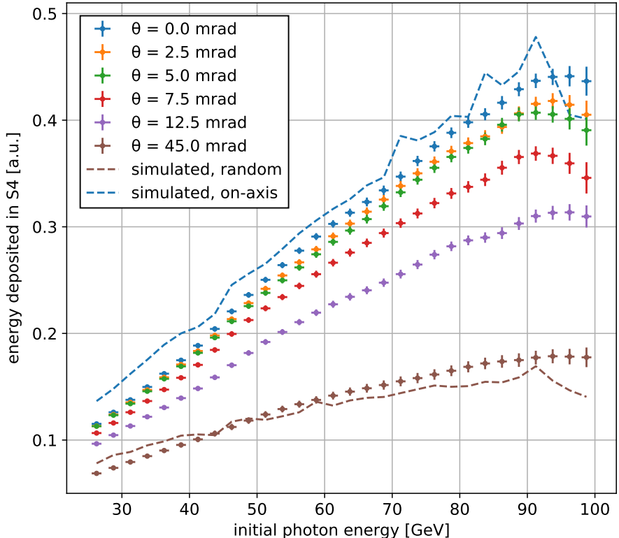
Fig. 3 Energy deposited in the S4 plastic scintillator as a function of the tagged photon energy, at different angles between the beam and the \langle 111 \rangle axis and in the random orientation (45 mrad). The points (dashed lines) represent the experimental data (simulated results).
