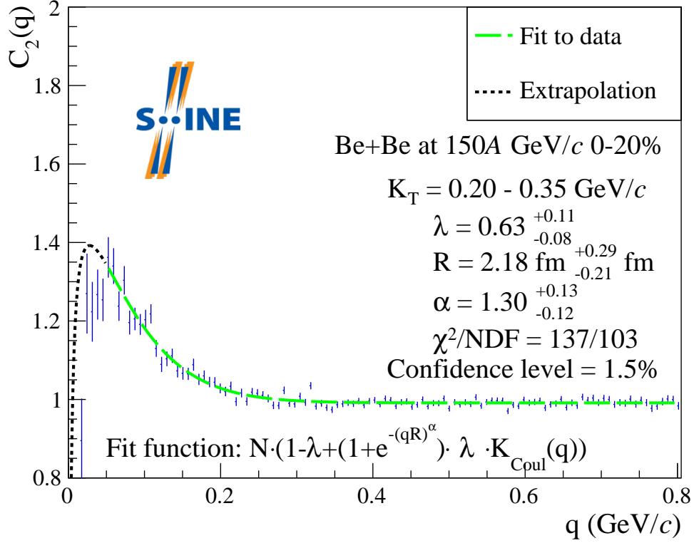
Figure 4: Example fit with Bose-Einstein correlation function at K_T = 0.20 - 0.35 \text{ GeV}/c for the sum (\pi^+ + \pi^+) + (\pi^- + \pi^-) . The green line shows the fitted function with Coulomb correction given by Eq. (16) within the range of 0.049 \text{ GeV}/c to 0.8 \text{ GeV}/c .
