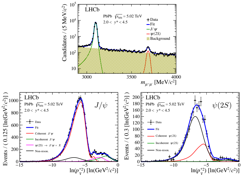
Fig. 1. Fit to the invariant mass distribution of dimuon candidates (top) and the \ln(p_T^{*2}) distribution fit of dimuon candidates within the 2.0 < y^* < 4.5 range for J/\psi candidates (bottom left) and \psi(2S) candidates (bottom right), where the starred notation indicates that the observable is defined in the nucleus–nucleus centre-of-mass frame.
