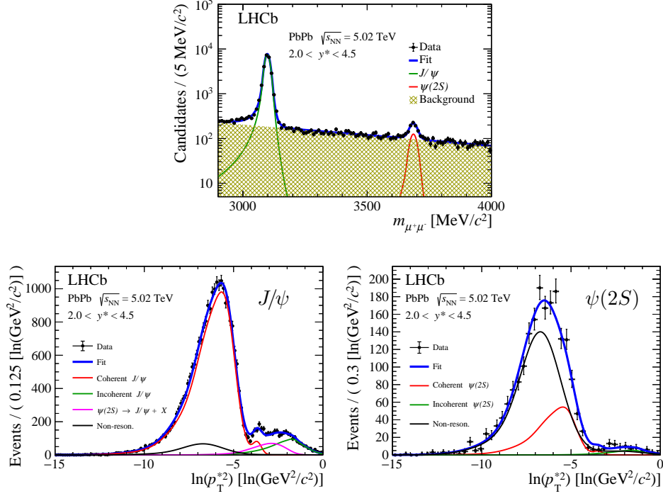
Fig. 1: Fit to the invariant mass distribution of dimuon candidates (up) and the \ln(p_T^*) distribution fit of dimuon candidates within the 2.0 < y^* < 4.5 range for J/\psi candidates (left) and \psi(2S) candidates (right), where the starred notation indicates that the observable is defined in the nucleus-nucleus centre-of-mass frame.
