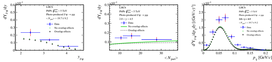
Fig. 5: The results of the differential photo-production yields of J/\psi versus the rapidity and the number of participants in collisions. Double-differential yields of the coherent J/\psi produced in peripheral PbPb collisions as a function of p_T (right).
