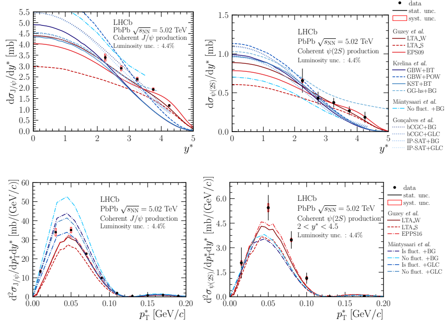
Fig. 2: Differential cross-section as a function y^* (up) and p_T^* (down) for coherent J/\psi (left) and \psi(2S) (right) production. Compared to theoretical predictions, which are grouped as perturbative-QCD calculations (red lines) and colour-glass-condensate models (blue lines).
