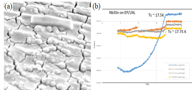
Figure 7: SEM plan view of Nb 3 Sn film (a) deposited at room temperature and annealed to 550 °C, (b) Critical transition temperature for film deposited at 650 °C.
