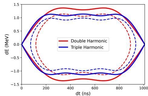
Figure 5: A comparison of the RF bucket shape (solid line) and bunch outline (dashed line) during double (red) and triple (blue) harmonic operation.
