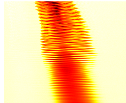
Figure 4: Longitudinal profile evolution during phase noise blow-up.
