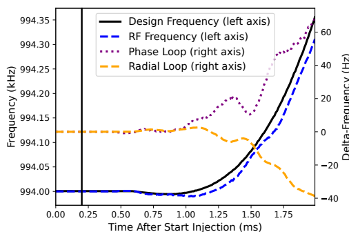
Figure 1: Design RF frequency, real RF frequency, and phase and radial loop corrections during the first 2 ms of a PSB cycle.
