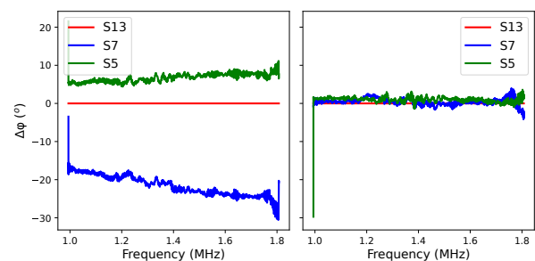
Figure 2: The change in measured beam phase when accelerating with a single cavity using Sector 13 as a reference.
