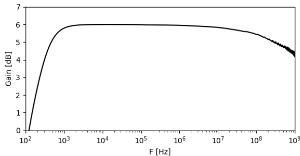
Figure 6: Bandwidth of the designed 25-kW combiner calculated using LTspice.
