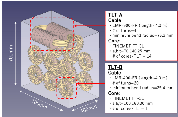
Figure 5: Overview of the 25 kW combiner.
