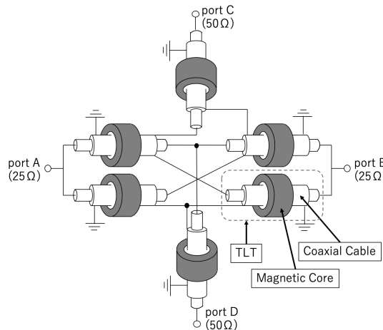
Figure 2: The configuration of the 2-way combiner [2].
