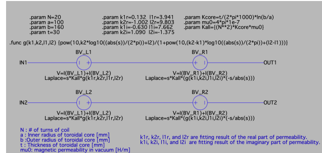
Figure 4: The toroidal core model considering the complex permeability with LTspice. Parameters shown in this figure are for FINEMET (FT-3L).
