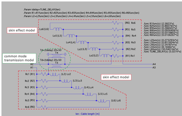
Figure 3: The coaxial cable model considering the skin effect and common mode signal propagation with LTspice. Parameters shown in this figure is for LMR-400-FR cable.
