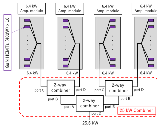
Figure 1: The configuration of 25-kW GaN amplifier.
