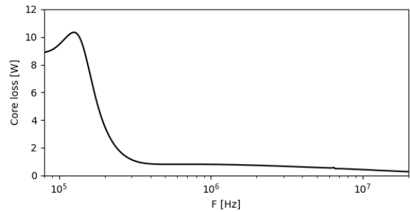
Figure 7: Core loss of the designed 25-kW combiner calculated using LTspice.
