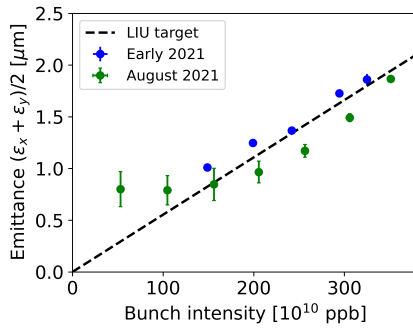
Figure 3: Emittance as function of intensity in the PSB early 2021 and August 2021. The brightness surpasses LIU project target values.
