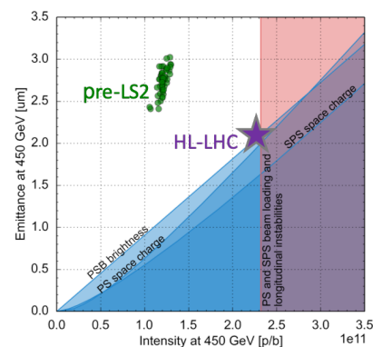
Figure 1: This plot shows the required emittance and bunch intensity for protons at the end of the injector chain. It corresponds to 2.3 \times 10^{11} protons per bunch in 2.1 \mu\text{m} emittance. These parameters have to be achieved for 288 bunches of 25 ns spacing. The measured performance before Long Shutdown 2 (LS2), before the LIU upgrades were installed, are shown in green. The parameter limitations of the different machines after the upgrade are indicated with the shaded regions.
