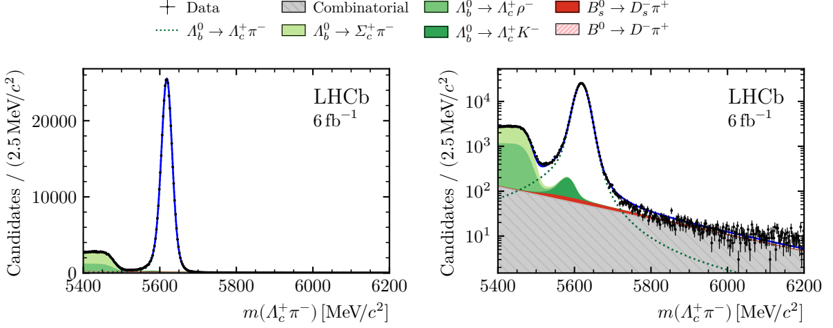
Figure 2: Invariant-mass distribution of \Lambda_b^0 \rightarrow \Lambda_c^+ \pi^- candidates, the normalisation channel in this measurement. The size of the signal peak compared to the backgrounds can be seen clearly in the linear plot on the left, whereas the individual components are displayed more clearly in the logarithmic plot on the right. Overlaid are the fit projections of the signal and background contributions, with individual components illustrated in the legend above.
