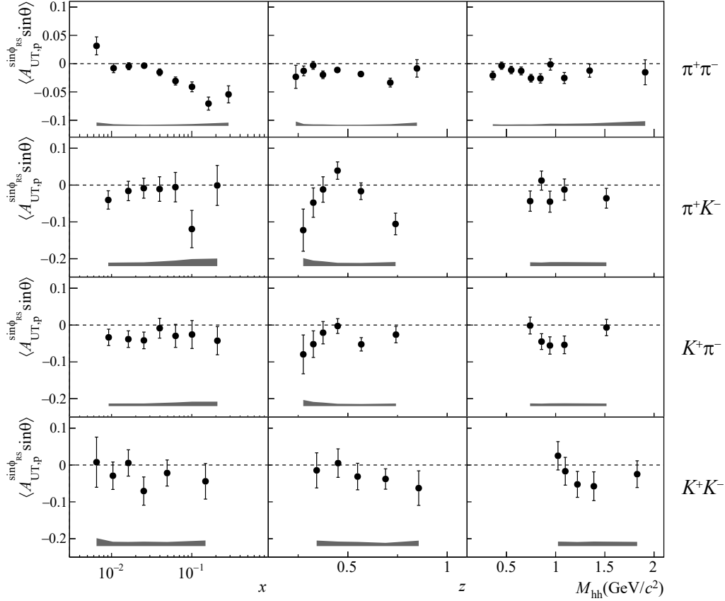
Fig. 3: Hadron-pair transverse-spin-dependent asymmetries as a function of x , z and M_{\text{hh}} , extracted from the full data set collected with the \text{NH}_3 (proton) target. Systematic uncertainties are shown by the gray bands.
