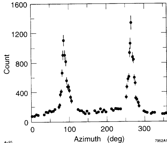
Figure 3. Azimuthal distribution of scattered He ion detected by the Ion-Scattering monitor in September 1994. This distribution corresponds to 1.6 \mu \times 80 nm spot.
