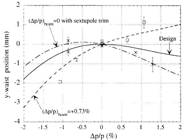
Figure 5. Shift of the vertical waist position as a function of the momentum offset of the incoming beam, measured at the Laser-Compton monitor. Squares are measured before the correction of the beam-energy offset. Dashed line is expected from the energy offset of +0.73\% . The crosses are measured after the correction. The dot-dashed is expected from the trimmed values then applied to the sextupoles. The design is shown by the solid line.
