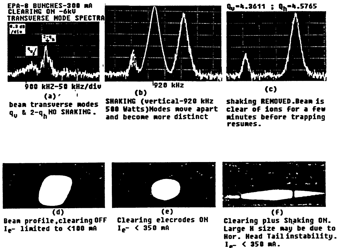
FIGURE 4 Beam profiles and transverse mode spectra with and without shaking on the CERN EPA machine.
