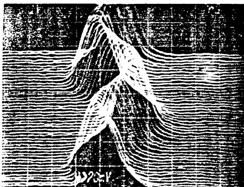
Synchrotronic oscillation (fs=3.84 kHz)
