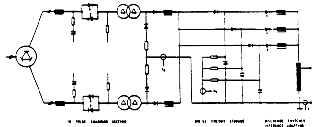
Fig. 1 - Circuit diagram of lithium lens pulser and power converter.
