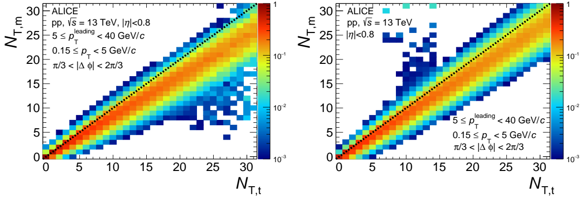
Figure 2: (Left) Correlation between the true N_{T,t} and the measured N_{T,m} multiplicity in the transverse region. (Right) Unfolding matrix M_{1_{tm}} . The iteration step of the unfolding matrix corresponds to the third.
