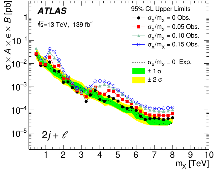
Figure 6: The 95% CL observed upper limits, in the m_{jj\ell} channel, on the cross-section times acceptance ( A ), efficiency ( \epsilon ) and branching ratio ( B ) for a Gaussian signal with various signal widths. The expected limit and the corresponding \pm 1\sigma and \pm 2\sigma bands are shown for \sigma_X/m_X = 0 signals. The limit for a width of 15% is shown starting from 0.75 TeV in order to avoid the region close to the minimum value of the m_{jj\ell} distribution.
