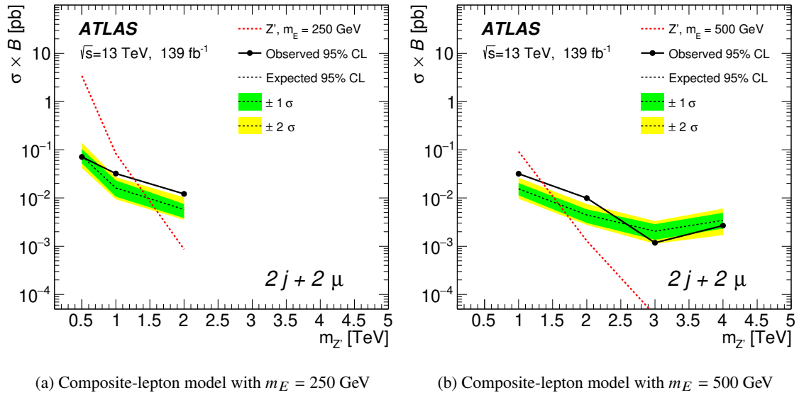
Figure 10: Observed (filled circles) and expected (dotted line with uncertainty bands) 95% CL upper limits on the cross-section ( \sigma ) times branching ratio ( B ) for Z' \rightarrow E\mu where the composite lepton E has a mass of (a) 250 GeV or (b) 500 GeV. The presented limits were obtained using the m_{jj\ell\ell} ( \ell = \mu ) distribution in events with at least one isolated muon with p_T^\ell > 60 GeV. Branching ratios of 100% to the final states of interest were assumed in the signal generation and computation of theory cross-sections. The black lines shown for the observed limits are provided to guide the eye.
