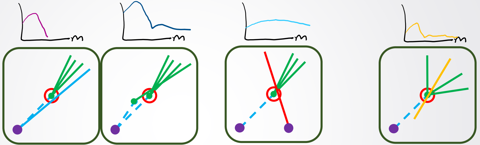
Crossed by track from same pp-interaction
