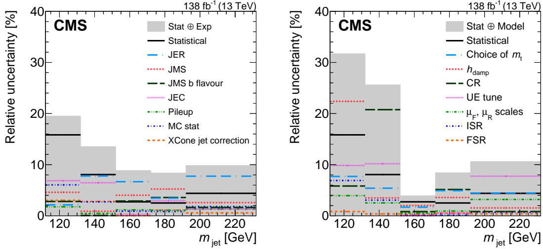
Figure 10: Relative experimental (left) and model (right) uncertainties after normalising the measurement to the total cross section. Various sources are displayed as coloured lines and compared to the total experimental or model uncertainty, respectively. The uncertainty sources are calculated as the square root of the diagonal entries from the respective covariance matrix, and do not include bin-to-bin correlations.
