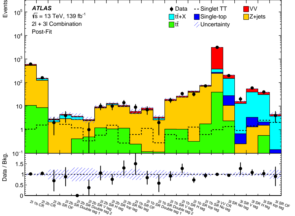
Figure 4: Summary of data and background yields in all analysis categories after the background-only fit. The expected yields for singlet T\bar{T} signal with m_T = 1.2 \text{ TeV} are also shown for comparison. The bottom panel shows the ratio of the data over the total background prediction. The shaded band includes statistical and post-fit systematic uncertainties.
