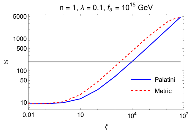
FIG. 4. Values of wormhole action as a function of \xi . The blue-solid and red-dashed lines are for the Palatini and metric formulations, respectively. The horizontal gray line shows a lower bound to solve the quality problem, S = 190 .
