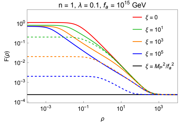
FIG. 1. F(\rho) for several values of \xi . The solid and dashed lines are for the Palatini and metric formulations, respectively.
