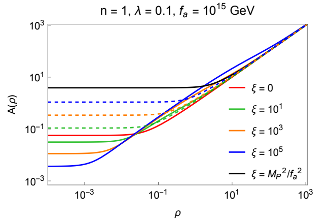
FIG. 2. A(\rho) for several values of \xi . The solid and dashed lines are for the Palatini and metric formulations, respectively.
