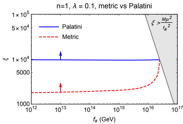
FIG. 5. f_a - \xi boundaries that marginally solve the quality problem in the Palatini (blue-solid) and metric (red-dashed) formulations. Regions above each line correspond to values that are safe from wormhole solutions spoiling the axion quality. The right gray region corresponds to values \xi > M_P^2/f_a^2 .
