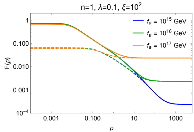
FIG. 6. F(\rho) for several values of f_a . The solid and dashed lines are for the Palatini and metric formulations, respectively.
