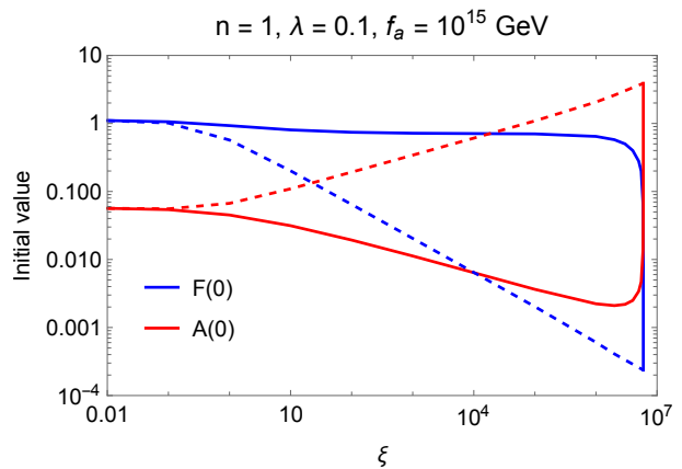
FIG. 3. F(0) and A(0) as functions of \xi . The solid and dashed lines are for the Palatini and metric formulations, respectively.
