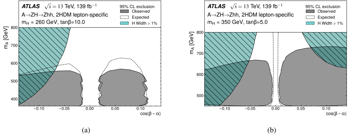
Figure 13: Interpretation of the upper limits on \sigma(A) \times B(A \rightarrow ZH \rightarrow Zhh \rightarrow Zbbbb) in the parameter space of the lepton-specific 2HDM. The same notation as in Figure 12 is used. Panel (a) refers to m_H = 260 GeV, \tan\beta = 10 and (b) refers to m_H = 350 GeV, \tan\beta = 5 .
