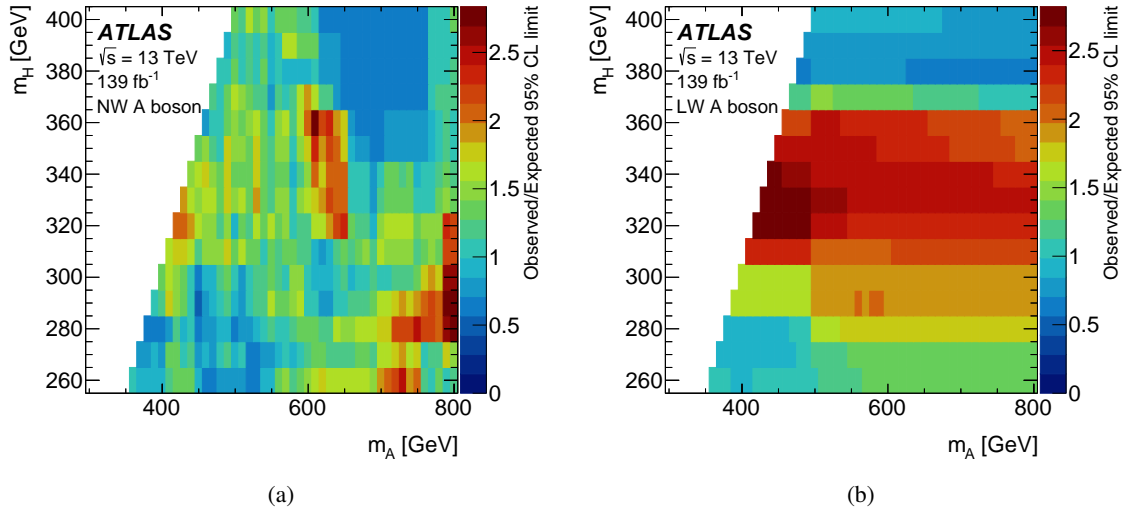
Figure 11: Ratios of the observed and the expected 95% CL upper bounds on \sigma(A) \times B(A \rightarrow ZH \rightarrow Zhh \rightarrow Zbbbb) in the (m_A, m_H) plane of the A \rightarrow ZH search with a (a) NW and (b) LW A boson. The A boson has a total decay width that is negligible compared to the experimental mass resolution in the NW case and is 20% of its mass in the LW case.
