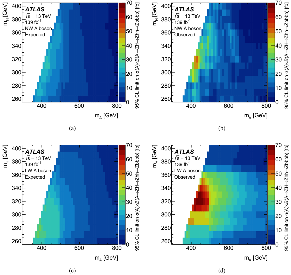
Figure 10: Upper bounds at 95% CL on \sigma(A) \times B(A \rightarrow ZH \rightarrow Zhh \rightarrow Zbbbb) in the (m_A, m_H) plane for (a, b) a NW A boson and (c, d) a LW A boson. The expected upper limits are shown in (a) and (c) while the observed limits are shown in (b) and (d). The A boson has a total decay width that is negligible compared to the experimental mass resolution in the NW case and is 20% of its mass in the LW case.
