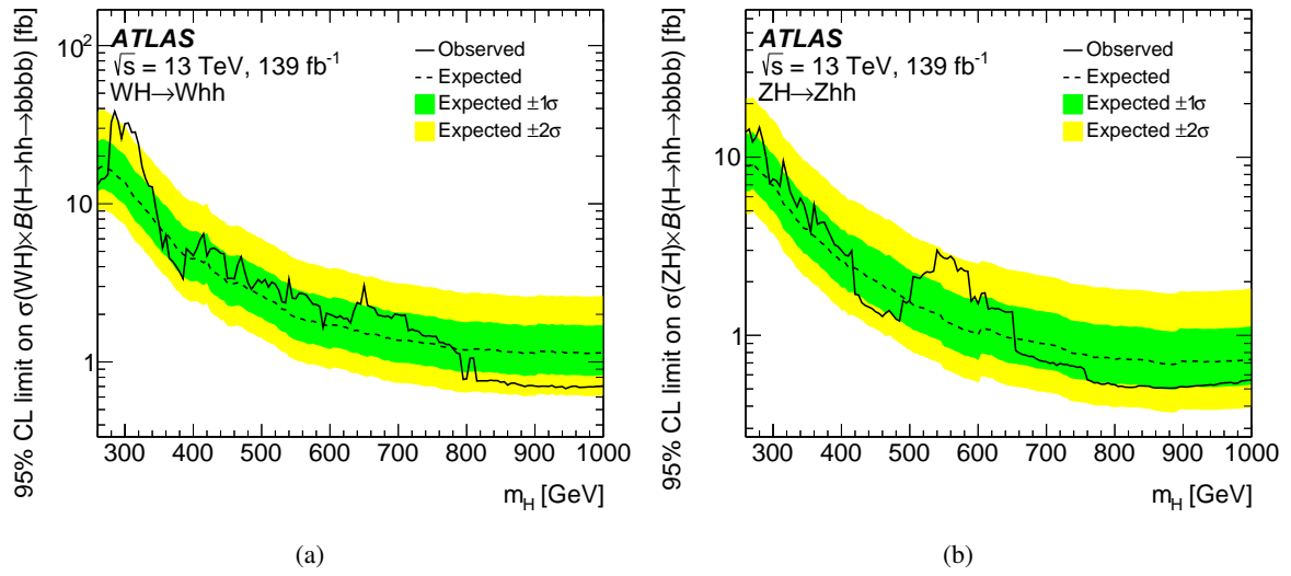
Figure 9: Observed (black solid curve) and expected (black dashed curve) 95% CL upper limits on the production cross-section at \sqrt{s} = 13 TeV of a heavy narrow scalar resonance H in the decay mode H \rightarrow hh \rightarrow bbbb in association with (a) a W boson and (b) a Z boson as a function of the resonance mass. The green (inner) and yellow (outer) bands represent \pm 1\sigma and \pm 2\sigma uncertainty in the expected limits.
