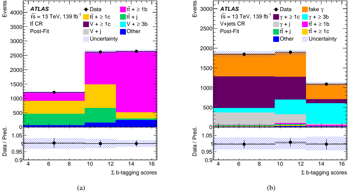
Figure 4: The background-only post-fit distributions of the sum of the pseudo-continuous b -tagging scores of the four jets with the highest scores in the (a) \text{CR}_{t\bar{t}} and (b) \text{CR}_{V+jets} control regions. The bottom panels show the ratios of the data to the total background expectations. The hashed bands represent the combined statistical and systematic uncertainties in the total background predictions.
