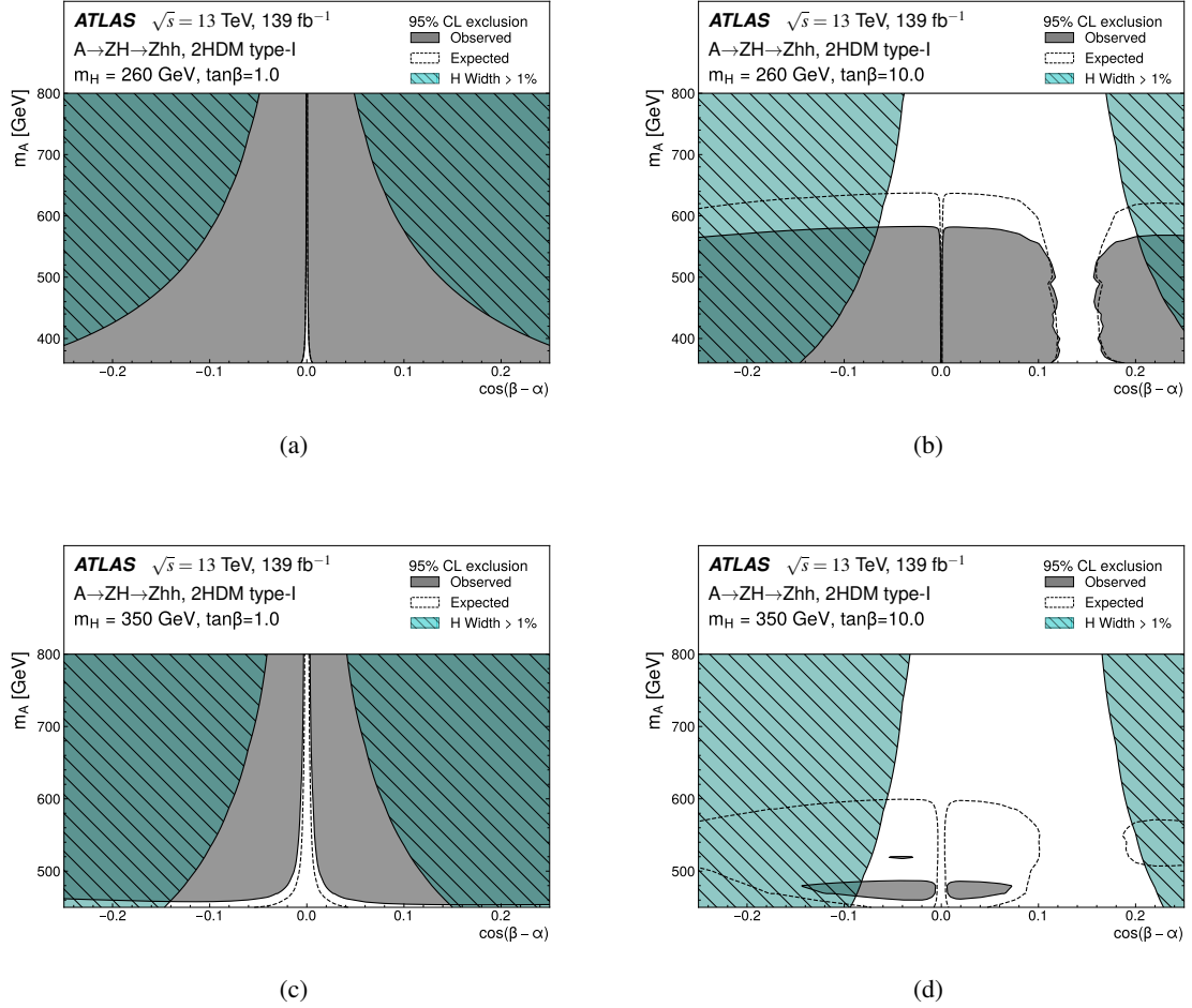
Figure 12: Interpretation of the upper limits on \sigma(A) \times B(A \rightarrow ZH \rightarrow Zhh \rightarrow Zbbbb) in the parameter space of the type-I 2HDM. The shaded areas correspond to 95% CL exclusion regions in the (\cos(\beta - \alpha), m_A) plane for a given m_H and \tan\beta . The hatched area corresponds to natural widths of the H boson for which the upper limits are not valid. Panels (a) and (b) refer to m_H = 260 GeV and to \tan\beta = 1 and 10, respectively; (c) and (d) refer to m_H = 350 GeV and to \tan\beta = 1 and 10, respectively.
