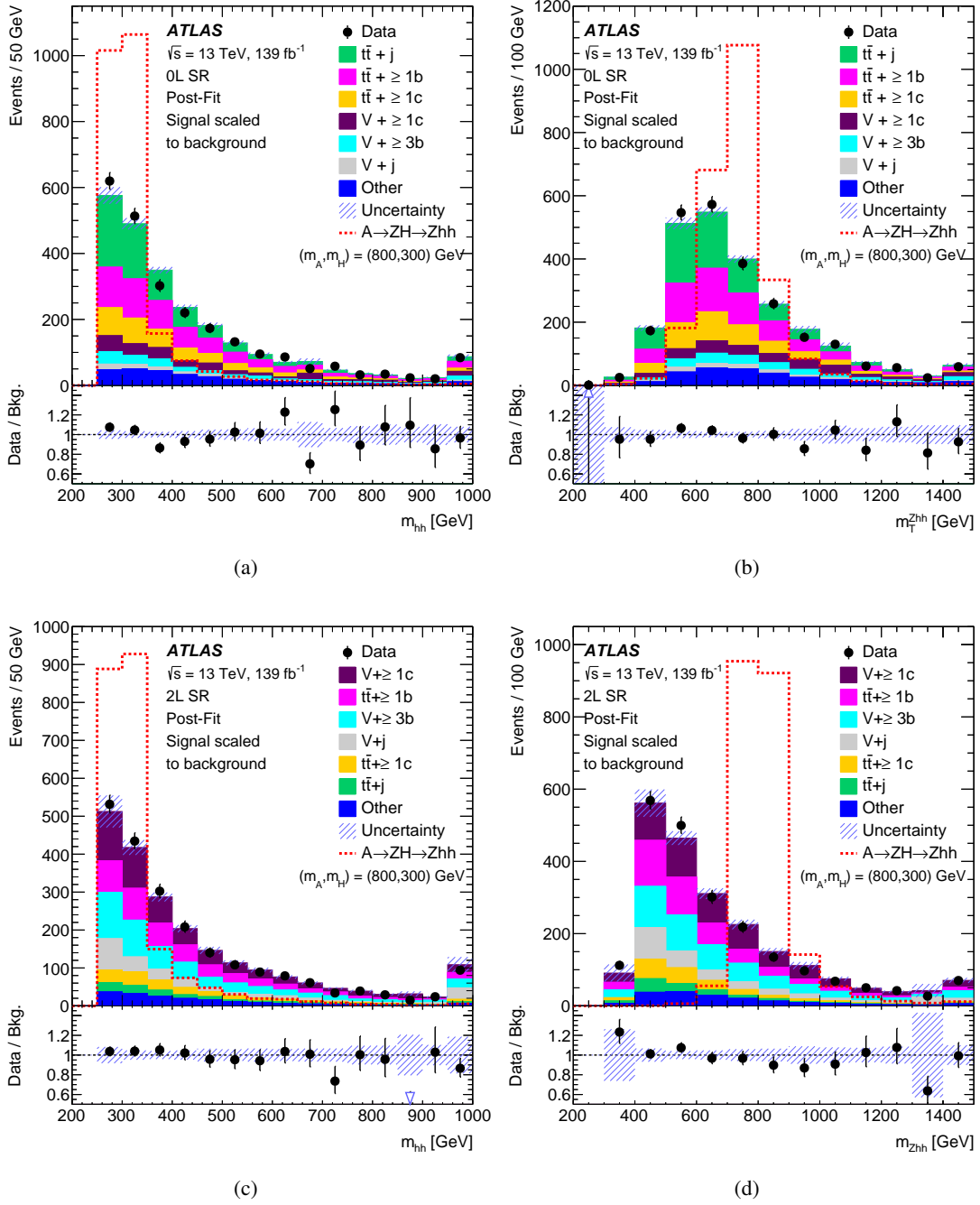
Figure 7: Comparisons between mass distributions of the data and the expected backgrounds: (a) m_{hh} and (b) m_{\text{T}}^{Zhh} of the 0L SR, and (c) m_{hh} and (d) m_{Zhh}^{Zhh} of the 2L SR. All masses are calculated after rescaling the measured Higgs boson candidate mass to 125 GeV. The backgrounds are obtained from the background-only fits to the control and signal regions discussed in Section 7. Expected distributions from the A \rightarrow ZH signal at (m_A, m_H) = (800, 300) GeV for a NW A boson, normalised to the total background expectations, are overlaid. The final bins include overflows. The bottom panels show the ratios of the data to the total background expectations. The hatched bands represent the combined statistical and systematic uncertainties in the total background predictions.
