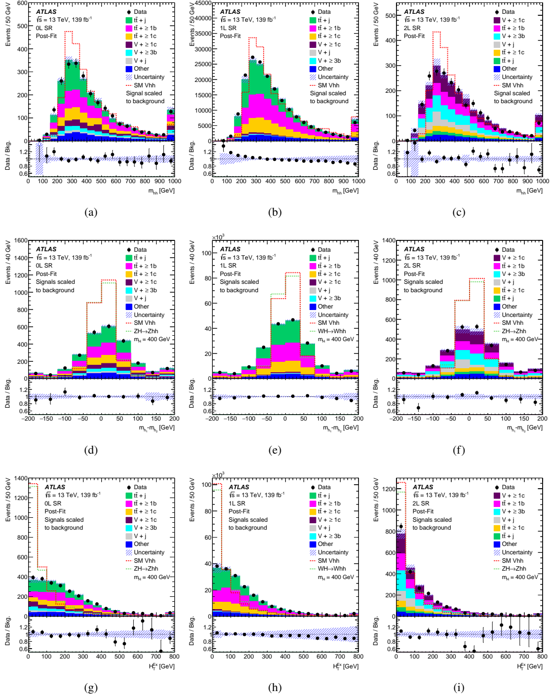
Figure 5: Example distributions of kinematic variables used in the BDT trainings: the invariant mass m_{hh} (a, b, c) and the mass difference m_{h_1} - m_{h_2} (d, e, f) of the two Higgs boson candidates, and H_T^{\text{ex}} (g, h, i) of events passing the 0L (a, d, g), 1L (b, e, h), and 2L (c, f, i) SR selections. The 1L SR combines 1L+ and 1L- categories. The expected distributions from example non-resonant and resonant signal models, normalised to the total background expectations, are overlaid. No resonant signal distributions are shown for m_{hh} , which is used in the BDTs for non-resonant production only. The final bins include overflows. The bottom panels show the ratios of the data to the total background expectations. The hatched bands represent the combined statistical and systematic uncertainties in the total background predictions.
