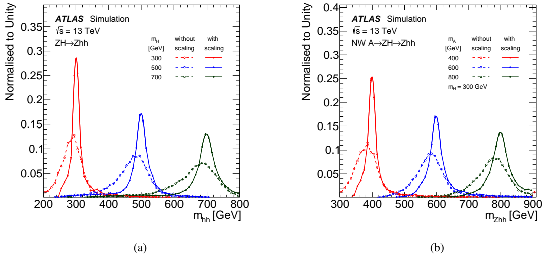
Figure 6: Reconstructed invariant mass distributions of (a) the hh system in the ZH search and (b) the Zhh system in the A \rightarrow ZH search with a NW A boson for a few representative signal mass points in the 2L channel. Distributions before the m_h rescaling are shown as open circles and dashed lines while those after the rescaling are shown as solid circles and solid lines. All distributions are normalised to unity. A NW A boson has a negligible total decay width compared with the experimental mass resolution.
