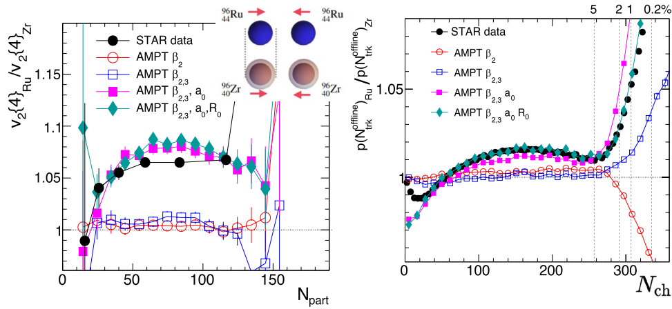
Fig. 5 (Color online) Ratios of observables taken between Ru+Ru and Zr+Zr collisions. The inset in the left panel shows how the neutron excess of ^{96}\text{Zr} compared to ^{96}\text{Ru} yields a more diffuse nuclear surface, i.e., a larger a_0 and a slightly smaller R_0 in Eq. (1). Left: the impact of the larger a_0 of ^{96}\text{Zr} manifests predominantly in the fourth-
