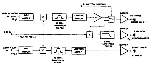
FIG. 2 - LOOP SIGNAL FILTERING
