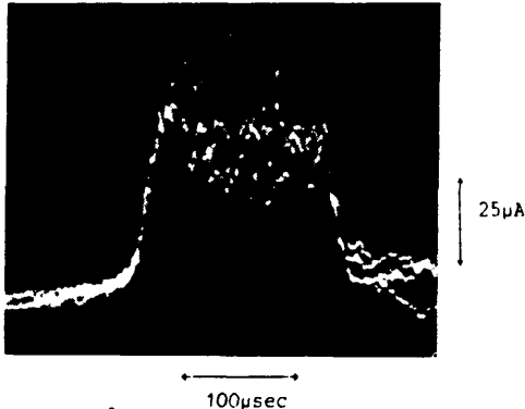
Fig. 6 : 0^8+ beam intensity measured in the LINAC-PSB line. 4 pulses superimposed
