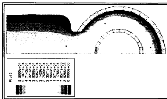
Figure 4: Simulation of the surface field distribution on the coupler iris using HFSS. The input waveguide comes from the left and the figure shows the first iris towards the disk-loaded waveguide.
