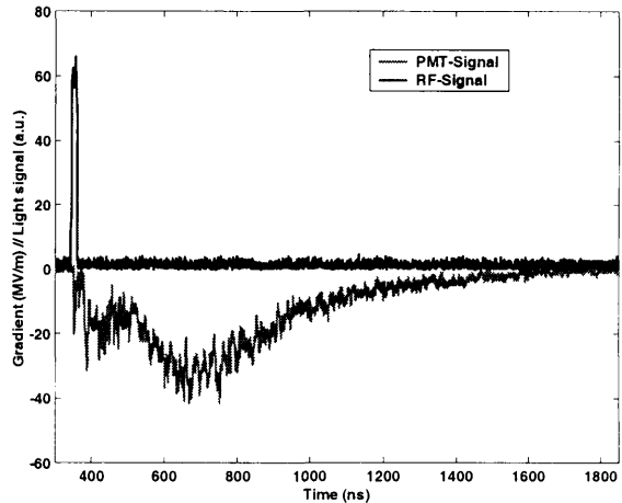
Figure 2: Visible light emission after a breakdown.
