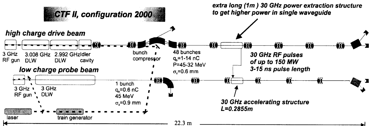
Figure 1: Configuration of CTF II in the year 2000 as a 30 GHz high-power test stand.
