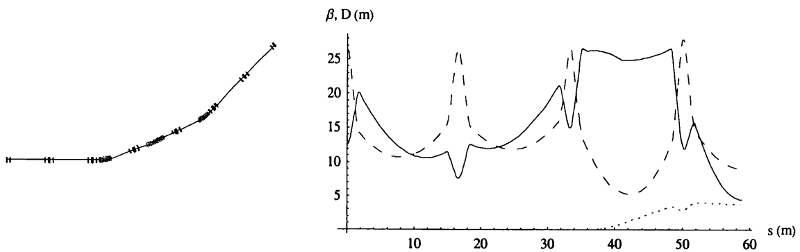
Fig. 1a: Structure of a Superperiod of the Accumulator
