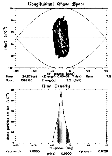
Figure 3b: Bunch after 7.5 Turns (End of Rotation) in the Compressor
