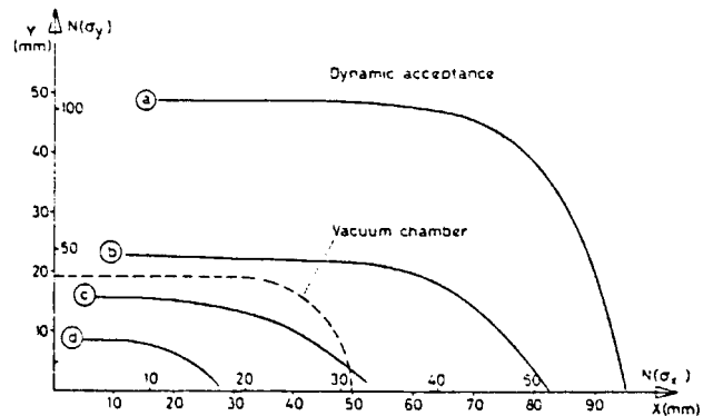
Fig. 3. Restriction of the EPA dynamic aperture with the sextupole component of the bending magnet at a) 0T/m, b) -2.8 T/m, c) -4.8 T/m and d) -7.2 T/m.
