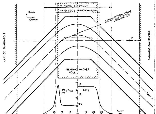
Fig. 1. Central trajectory and max beam envelope in the EPA bending magnet computed from calculated magnetic field B and orthogonal gradient dB/dx .
