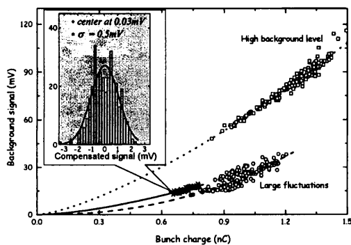
Figure 3: Background signal as a function of bunch charge
