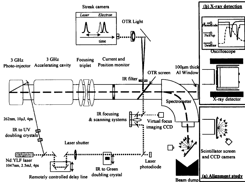
Figure 1: Laser Wire Scanner experimental layout on CTF2
