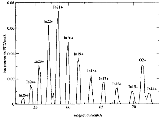
FIG. 2 Indium charge state distribution (2.5 keV/u).
