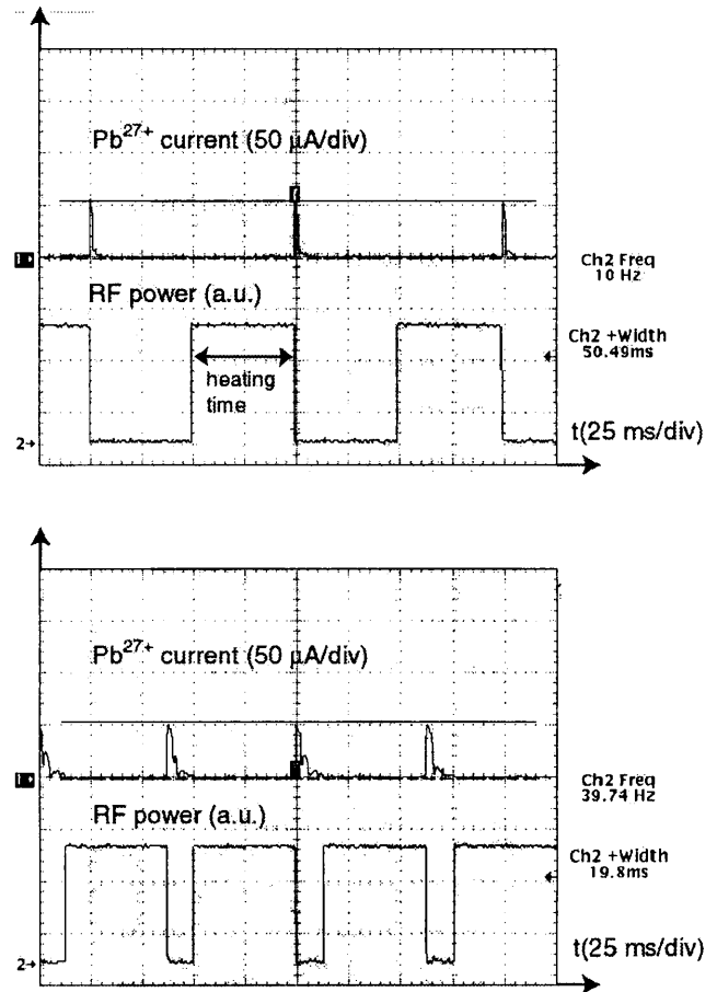
FIG 3. Effect of heating time and repetition rate for Pb^{27+} . Upper trace, beam current, lower trace RF power. Repetition rate is indicated by Ch2 Frequency.
