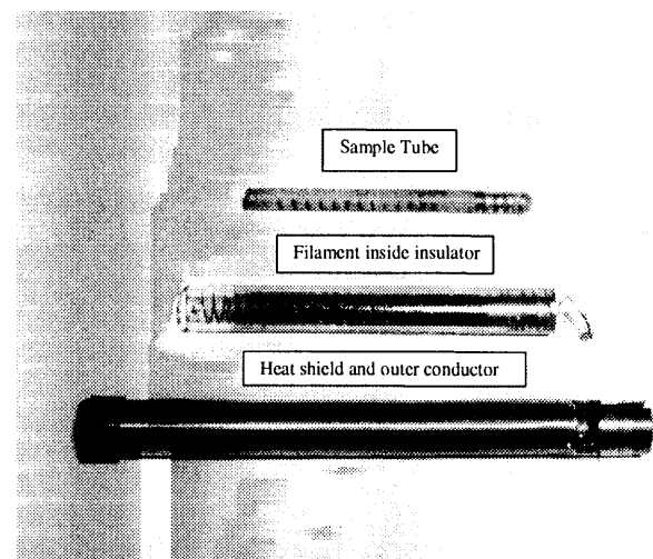
FIG. 1 The oven used for lead or indium.
