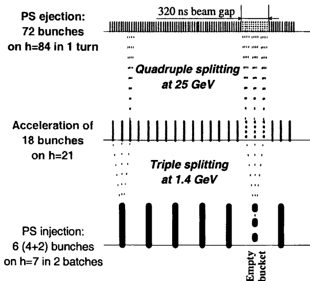
Figure 5: Multiple splitting scheme for the LHC beam.
