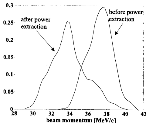
Figure 4: Drive beam momentum spectra measured before and after the 30 GHz power extraction structures.
