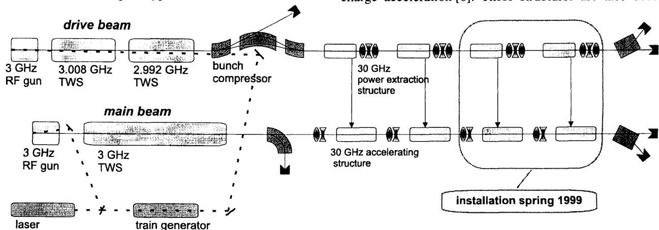
Figure 1: Layout of CTF II (TWS=travelling wave structure)
