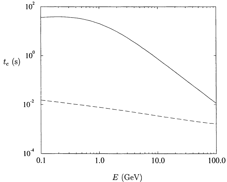
Fig. 6. The long cooling time approximation is valid when t_c is much larger than the values shown by the solid line above, while the short cooling time is valid far below the dashed line. There is thus a large interval where none of these approximations is valid.
