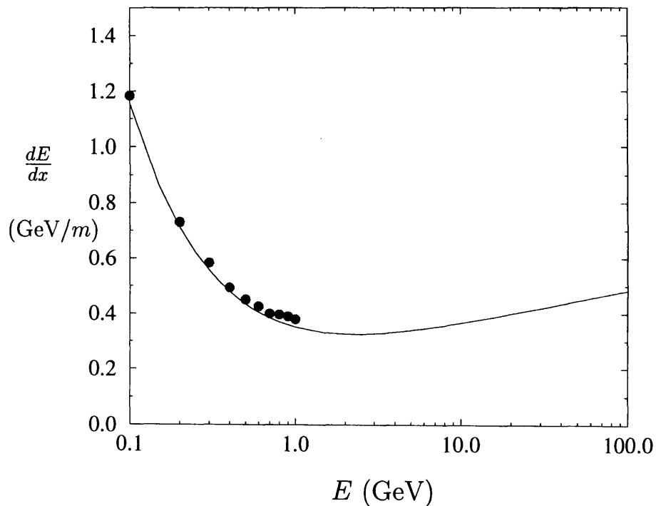
Fig. 2. Simulated and Bethe–Bloch values of dE/dz for a carbon wire as a function of kinetic energy, E = m_p c^2 (\gamma - 1) .
