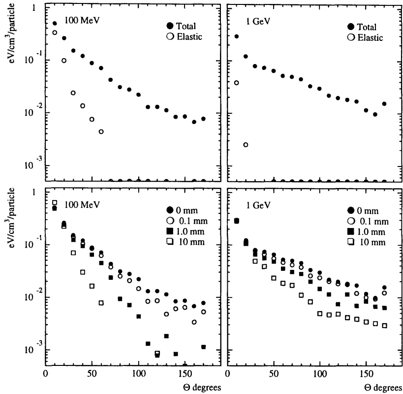
Fig. 3. Energy deposition in the polyethylene detectors as a function of angle with respect to the beam direction. Normalisation is to one particle incident on the 30 \mu\text{m} wire.
