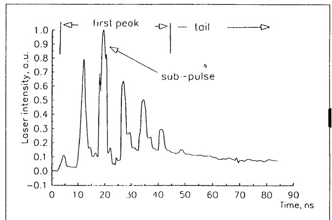
Fig.3. Pulse Shape of a Self locking Laser.
