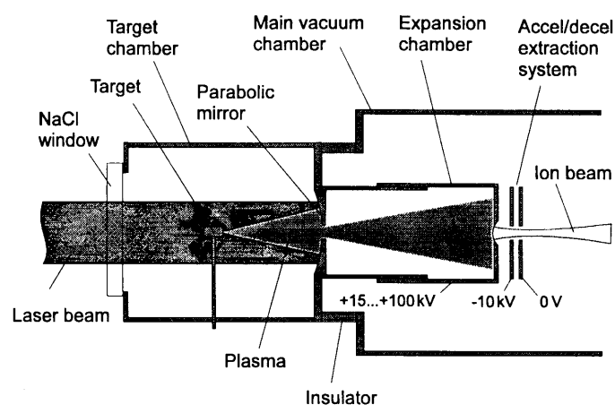
Fig.1. Configuration of a Laser Ion Source
