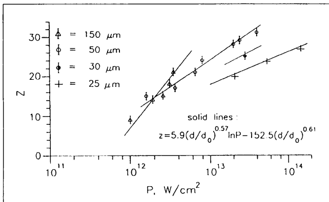
Fig.2. Charge-State as Function of Power Density ( d_0 = 50 \mu\text{m} ).
