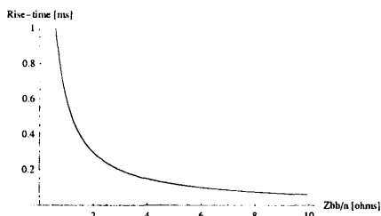
Figure 4: Microwave-instability rise-time (neglecting Landau damping) for the macro-bunch at the end of the accumulation process vs. Z_{bb}/n .
