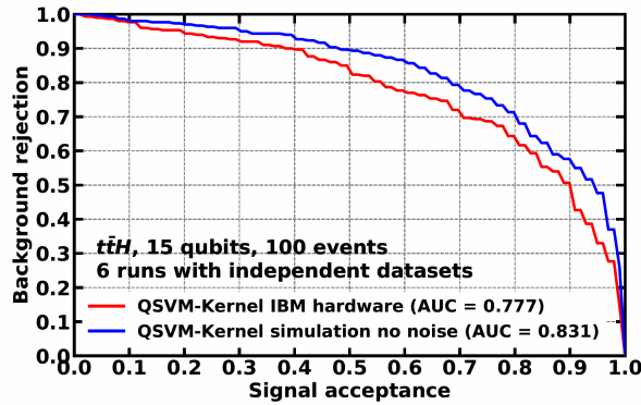
Figure 5: ROC curves of the QSVM-Kernel classifier with the “ibmq paris” quantum computer hardware and the noiseless quantum computer simulator using the t\bar{t}H analysis datasets of 15 qubits and 100 events.
