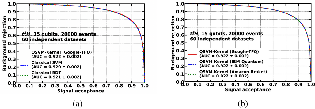
Figure 4: ROC curves of various classifiers in the t\bar{t}H analysis using 15 qubits and 20000 events. Each curve represents results averaged over 60 statistically independent datasets.
