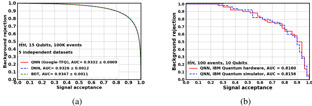
Figure 6: ROC curves of various classifiers using the t\bar{t}H analysis datasets of 100000 events and 23 input variables (a), ROC curves of the QNN classifier with the “ibmq paris” quantum computer hardware and IBM quantum computer simulator using the t\bar{t}H analysis datasets of 100 events (b).
