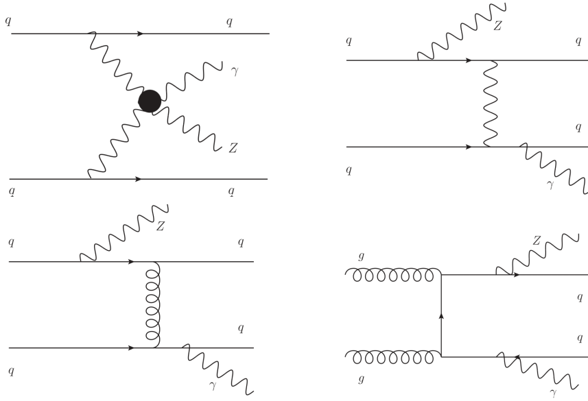
Figure 1: Feynman diagrams of electroweak Z\gamma jj production involving the VBS subprocess (top left) or non-VBS subprocesses (top right) and of QCD Z\gamma jj production with gluon exchange (bottom left) or the s-channel gg\text{--}qq process (bottom right).
