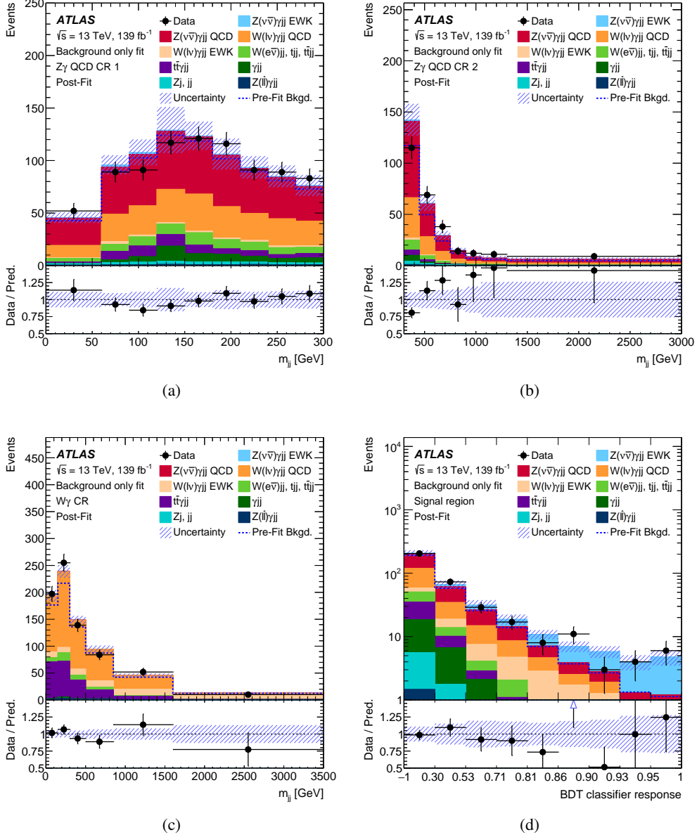
Figure 4: The m_{jj} distributions for the (a) Z\gamma QCD CR 1, (b) Z\gamma QCD CR 2, and (c) W\gamma CR, and the BDT classifier response distribution for the (d) SR after the fit in all regions. The BDT classifier response was remapped into equal-width bins for better representation. The dashed line shows the total background distribution before the fit. The vertical error bars on the data points correspond to the data's statistical uncertainty. Overflows are included in the last bin. The lower panel shows the ratio of observed to expected event yields. The uncertainty band corresponds to the combination of the statistical and systematic uncertainties obtained in the fit.
