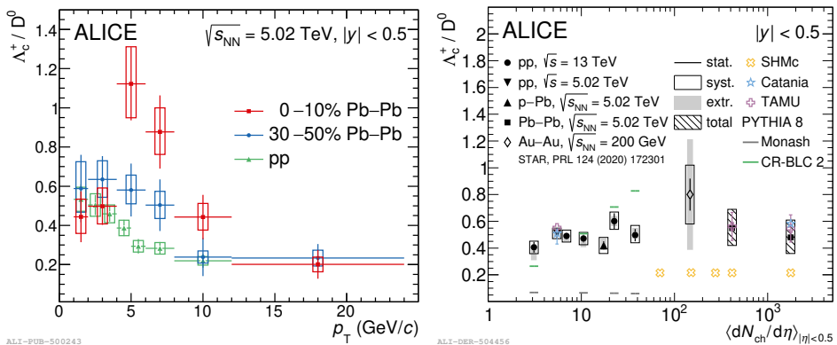
Fig. 3. Left: the \Lambda_c^+/D^0 yield ratio in central and mid-central Pb–Pb collisions [7] compared with the result from pp collisions [13]. Right: the p_T -integrated \Lambda_c^+/D^0 ratios as a function of multiplicity in pp , p -Pb, Au–Au, and Pb–Pb collisions [7, 13, 15] compared with theoretical predictions [16].
