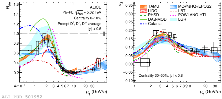
Fig. 1. The average R_{AA} (left) and v_2 (right) of prompt D^0 , D^+ , and D^{*+} mesons in, respectively, the 0–10% and 30–50% centrality classes [4] compared with predictions of charm-quark transport models [11].
