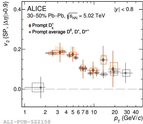
Fig. 2. The v_2 of prompt D_s^+ in the 30–50% centrality interval [6] compared with that of non-strange D mesons [5]. The systematic uncertainty due to the feed-down subtraction is shown separately as shaded boxes.
