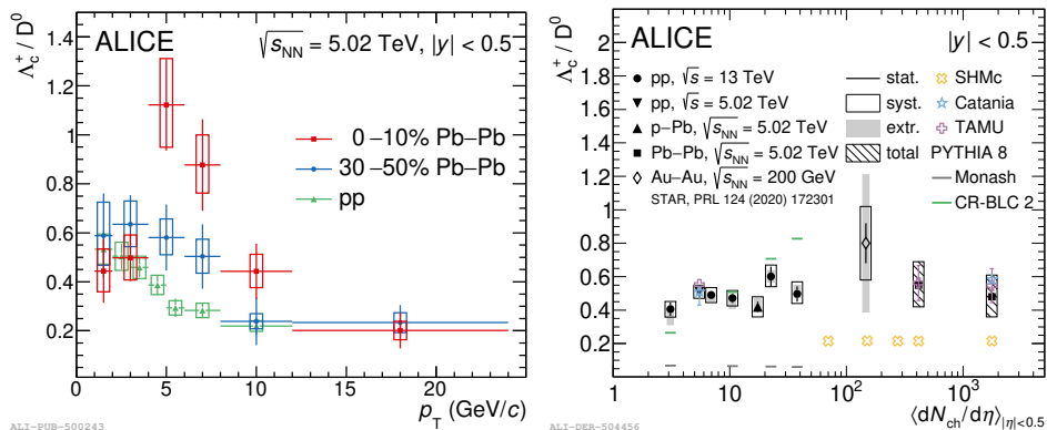
Fig. 3. Left: the \Lambda_c^+/D^0 yield ratio in central and mid-central Pb–Pb collisions [7] compared with the result from pp collisions [13]. Right: The p_T -integrated \Lambda_c^+/D^0 ratios as function of multiplicity in pp, p–Pb, Au–Au, and Pb–Pb collisions [7, 13, 15] compared with theoretical predictions [16].
