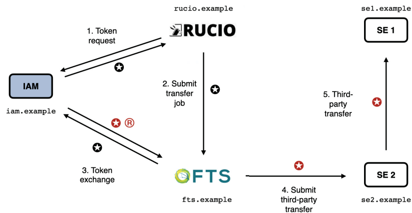
Figure 1. Token flows used in the RUCIO managed data-transfer scenario.
